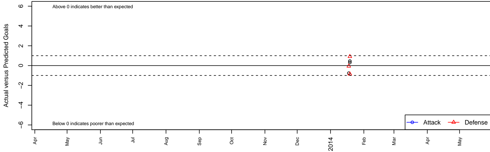
Impact Black B99 Dots are actual minus expected GF (blue circles) and GA (red triangles). Blue line is smoothed change in attack strength. Red is smoothed change in defense strength.
